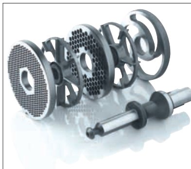
5 part cutting set MC 3-1 / MC 3-2
